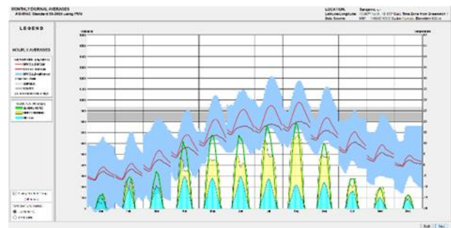
Figure 6. Average temperature values and solar radiation values for Sarajevo (Source: authors)
