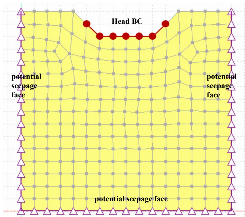
Figure 3. Layout of finite element mesh and boundary conditions used
