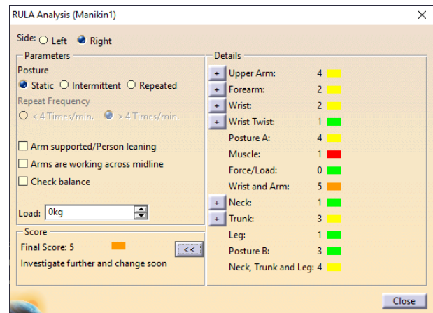
Figure 3. Results of the Rula analysis for the case m=70 kg and the slope of the workbench \alpha=20^0
