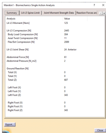
Figure 2. Results of biomechanical analysis for m=70 kg and the slope of the workbench \alpha=20^0
