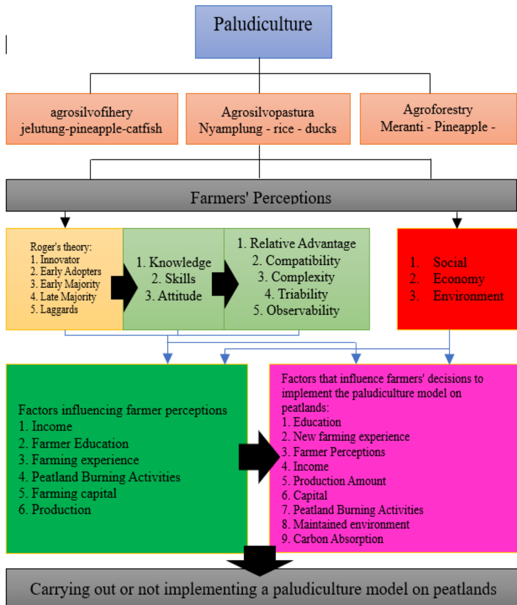
Figure 2. Research flow
