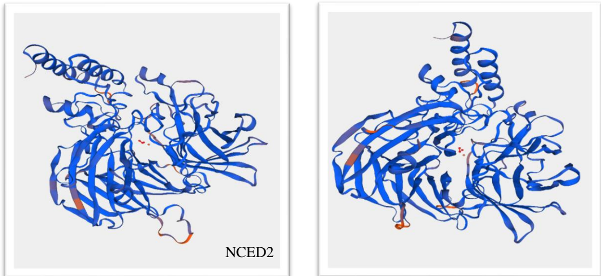
Figure 3. Predicted 3D structures of NCED 2 and NCED 3 proteins
